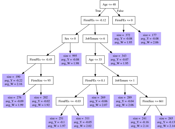
Figure C.1: Example of decision tree
