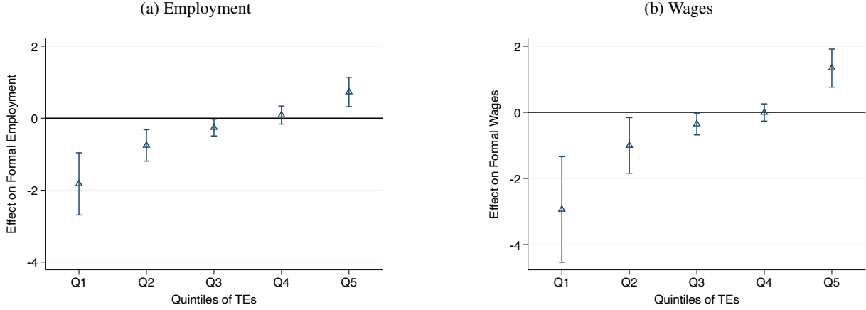
Figure B.6: Quintiles of treatment effects for formal employment and formal wages in the causal forest, 2015–2018
