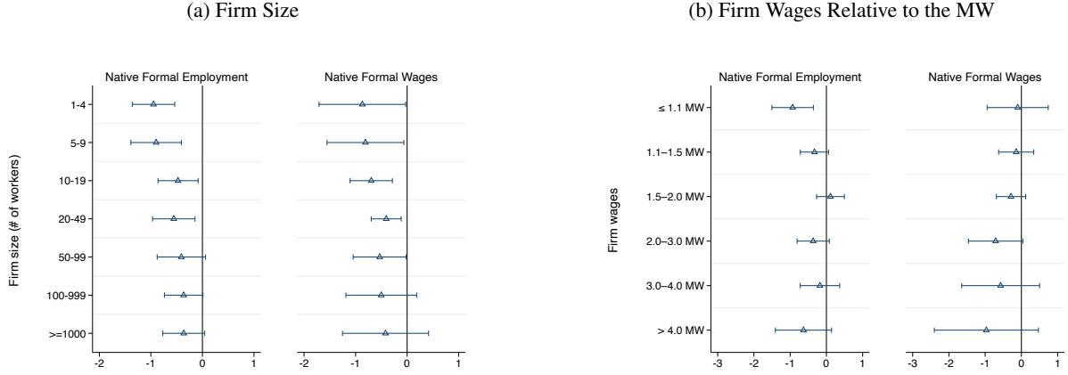
Figure 5: Employment and wage estimates, 2015–2018
