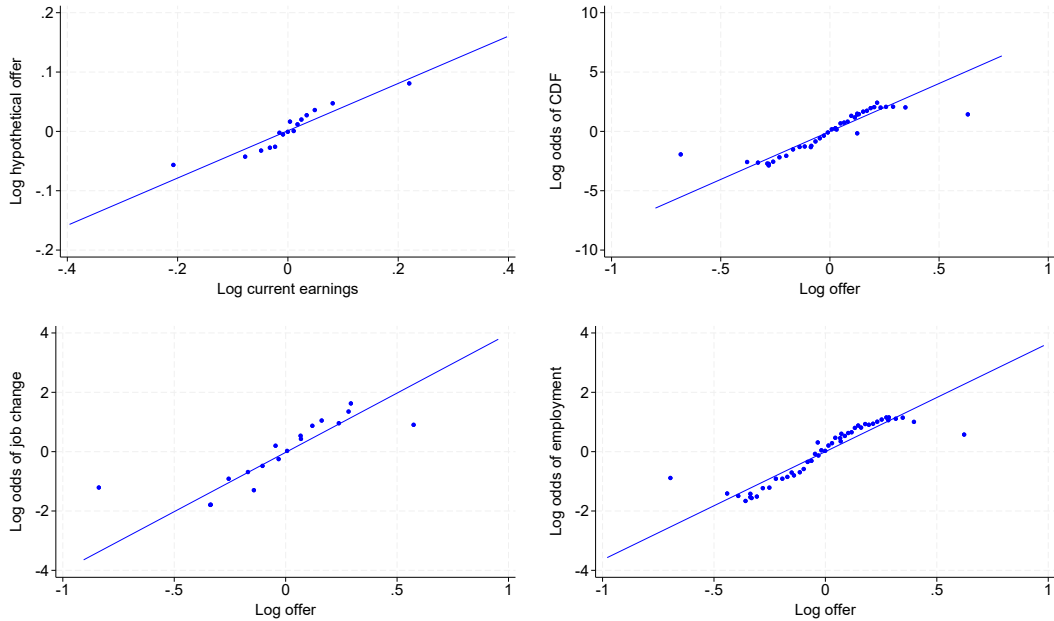
Figure 3: Key elements for model identification. Binned scatter plots (randomized quantile bins) with overlaid linear fits estimated on the raw data. All variables are demeaned. Top left: persistence — log expected best offers on log current earnings. Top right: risk — log odds of the subjective CDF of expected offers plotted against log offer. Bottom left: log odds of changing employer (conditional on employment) by log offer. Bottom right: log odds of becoming employed (conditional on unemployment) by log offer. The log offer corresponds to the log midpoint of each elicited offer bin, defined as a multiplicative factor of the individual's expected best offer.
