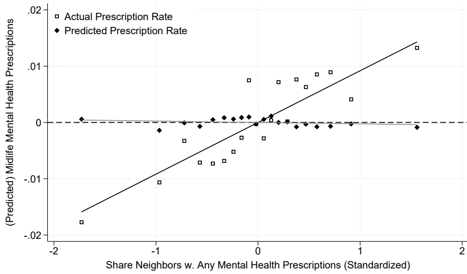
Figure 5: Local Mental Health Treatment Intensity - Relevance and Balance
